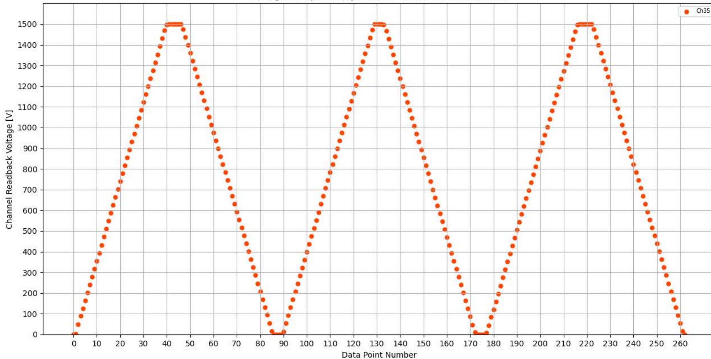
Voltage Ramp Test (Python) Bd #316, Slot #0, Ch #35
